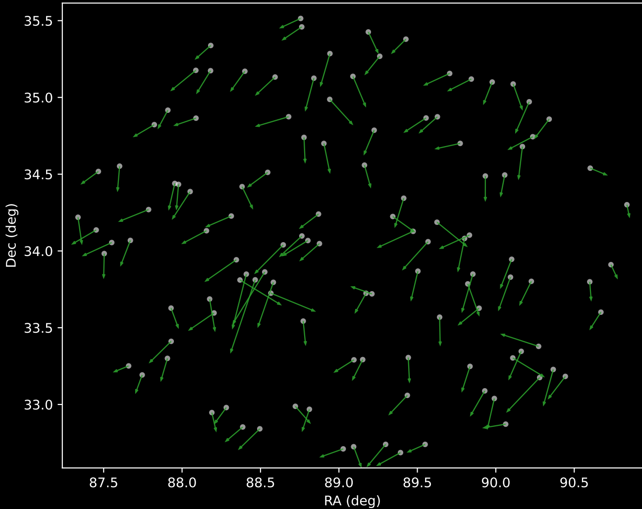
APOGEE DR17 Cluster 4 Proper Motion Vectors (n=117)
