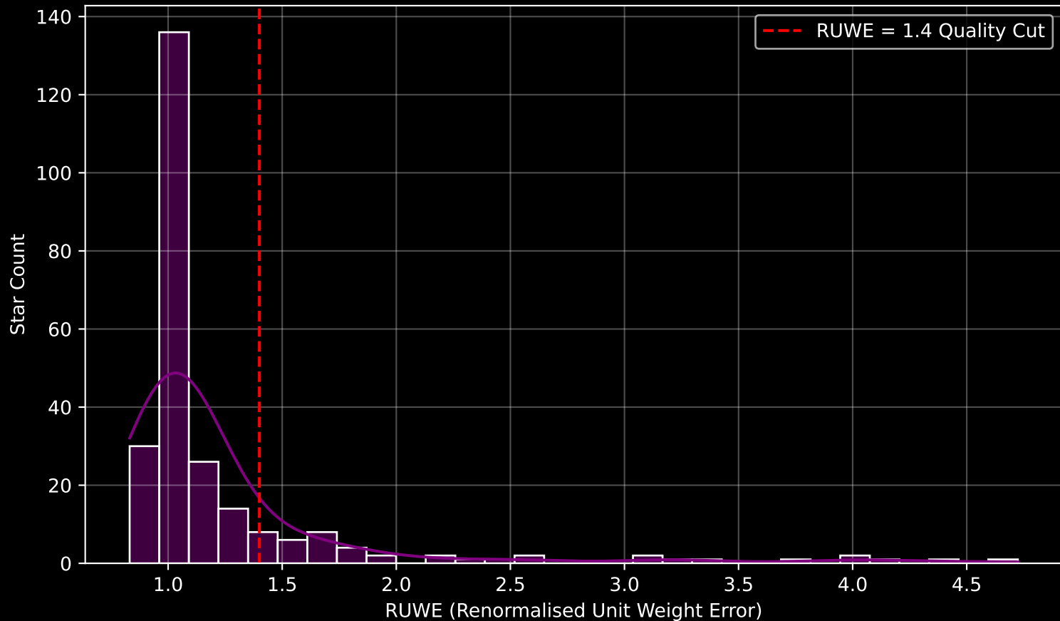
GAPOGEE DR17 Field [101-24_btx] RUWE Distribution (n= 250)
