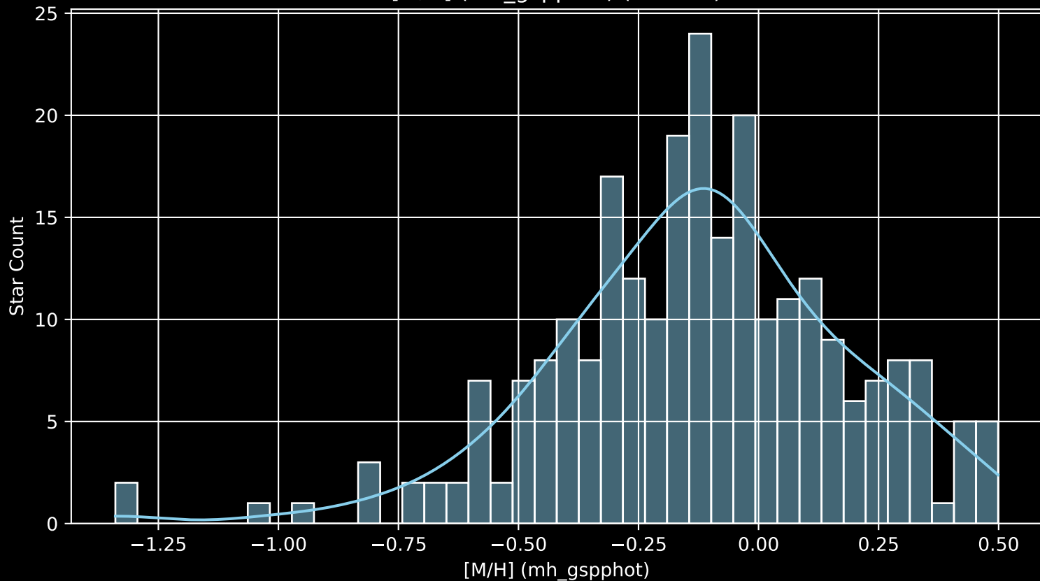
APOGEE DR17 Field: [101-24_btx [M/H] (mh_gspphot) (n= 253)
